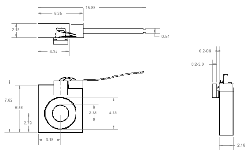
C-Mount Package
