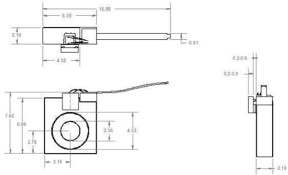
C-Mount Package
